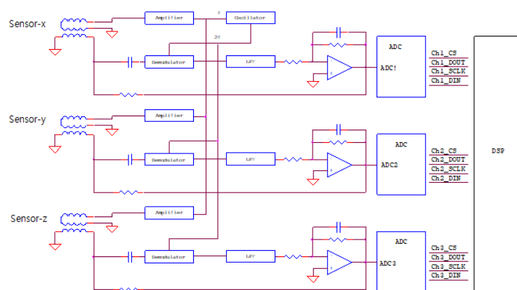
Fig. 1. Schematic diagram of 3-axis simultaneous measuring flux-gate magnetometer for scalar magnetometer.
