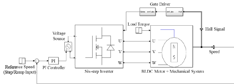
Fig. 2. Inverter simulation for BLDC control
