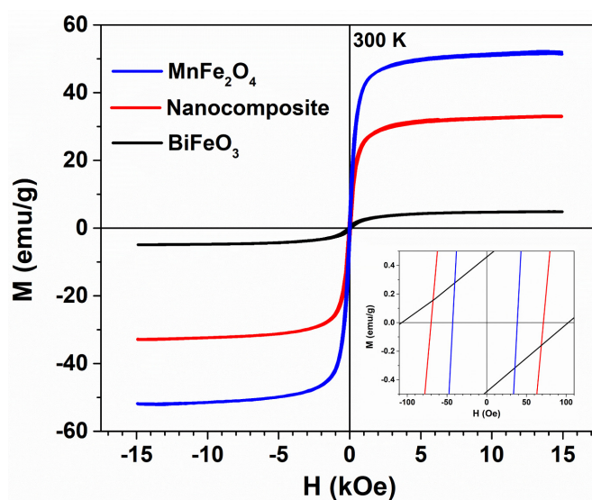
Fig. 1. M-H loops of BFO, MFO and their nanocomposite measured at 300K. The inset shows the magnification at low field strength
