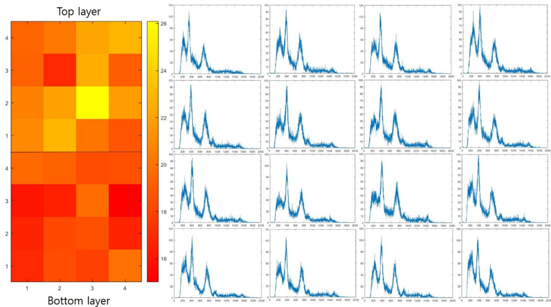
Fig. 1. Energy resolution distribution (left) and energy spectra (right) corresponding to each pixel position in the flood image
