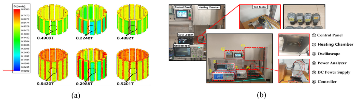
Fig. 1. reliable analysis of synchronous motors with permanent magnets, (a) demagnetization analysis based on 3D model (b) Experiment of demagnetization
