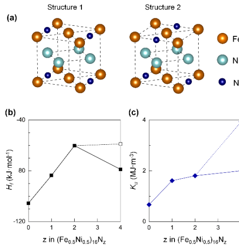
Fig. 1. (a) Possible distribution patterns of the interstitial N atoms, (b) formation enthalpy and (c) uniaxial magnetic anisotropy of structures.
