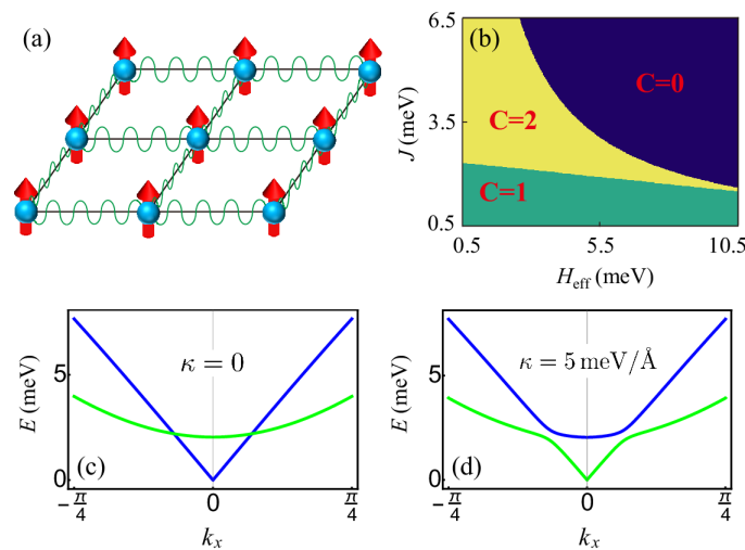
Fig. 1. (a) The schematic illustration of the magnon and phonon system. (b) The Chren number of the magnon-phonon system. H_{\text{eff}} represents the effective magnetic field including the anisotropy field and the external magnetic field.
