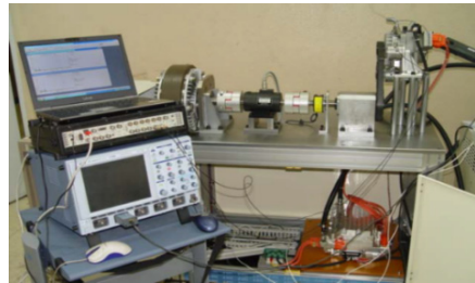
Fig. 4. Experimental set-up.
