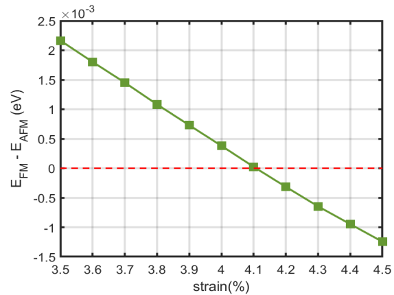
Fig. 2. Energy difference between FM and AFM state of bilayer FGT, \Delta E = E_{\text{FM}} - E_{\text{AFM}} , with respect to strain.
